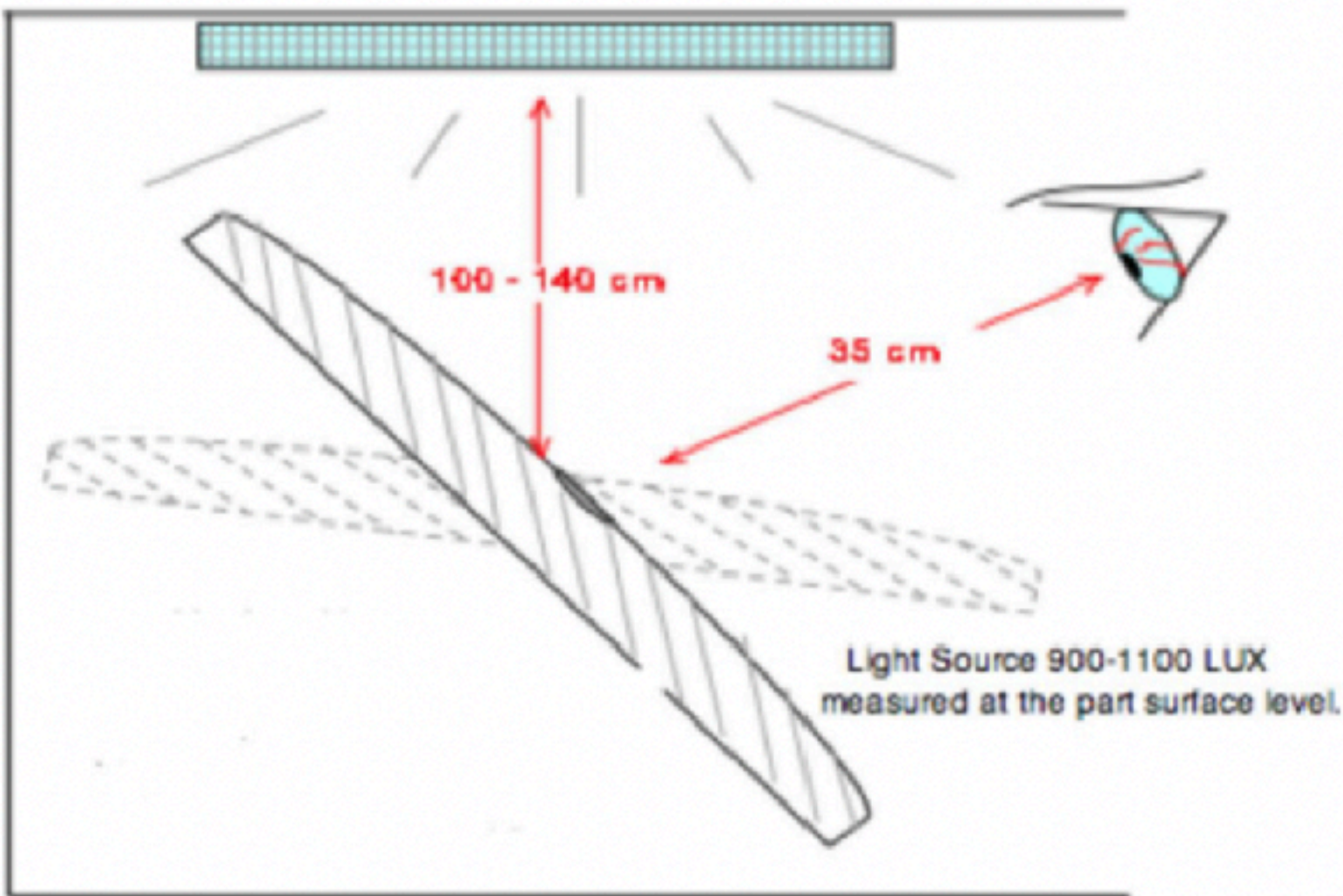
Fig. 1 Inspection criteria for opaque surfaces / all classes
